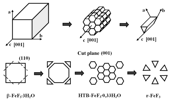
Fig. 8. Model of structural transformations at the dehydration of the obtained material \beta\text{-FeF}_3 \cdot 3\text{H}_2\text{O}
