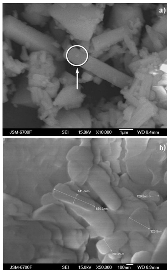
Fig. 3. Microscopic images of the obtained \beta - \text{FeF}_3\cdot 3\text{H}_2\text{O} material
