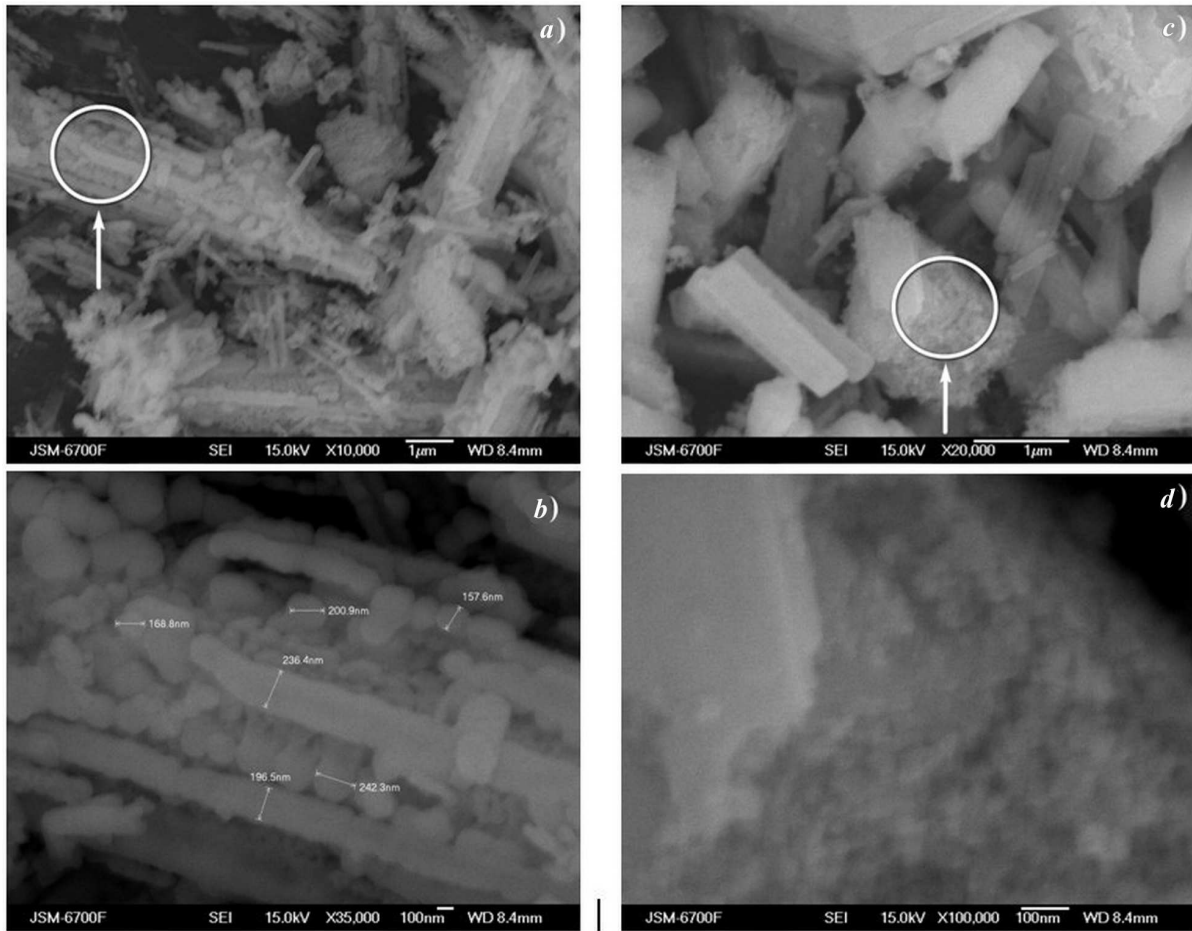
Fig. 7. Microscopic images of the obtained materials: HTB- \text{FeF}_3 \cdot 0.33\text{H}_2\text{O} (a and b) and r- \text{FeF}_3 (c and d)
