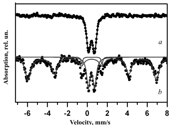
Fig. 6. Mössbauer spectra of HTB-FeF 3 ·0.33H 2 O (a) and r-FeF 3 (b)
