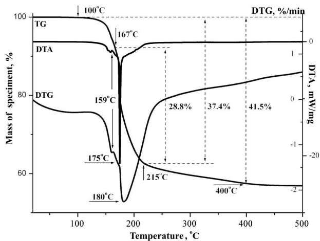
Fig. 4. TG, DTG, and DTA curves for the synthesized \beta - \text{FeF}_3\text{3H}_2\text{O} material
