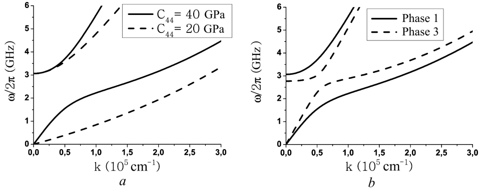
Dispersion laws for magnetoelastic waves: (a) in the ground state \mathbf{H} \parallel \mathbf{M} \parallel \langle 001 \rangle for two values of elastic modulus C_{44} and (b) in the ground state \mathbf{H} \parallel \mathbf{M} \parallel \langle 101 \rangle and \mathbf{H} \parallel \mathbf{M} \parallel \langle 111 \rangle for C_{44} = 40 GPa
