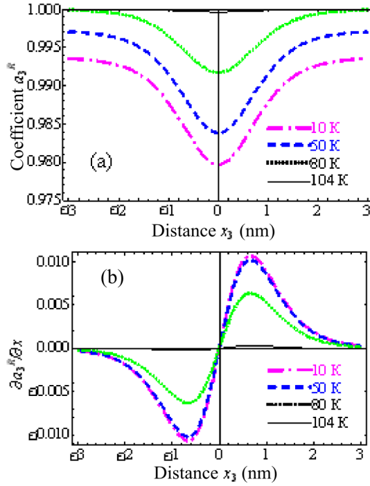
Fig. 2. Spatial distributions of (a) the coefficient a_3^R normalized by its maximum value and (b) its derivative with respect to the coordinate at various temperatures
