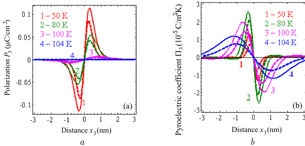
Fig. 3. Analytical (solid curves) and numerical (dashed curves) spatial distributions of (a) the polarization component P_3 and (b) the pyroelectric coefficient \Pi_3 at various temperatures
