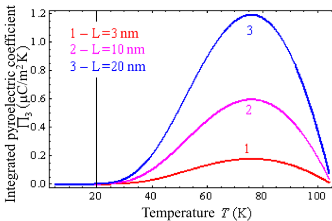
Fig. 4. Dependences of the integrated pyroelectric coefficient on the temperature at various averaging intervals L
