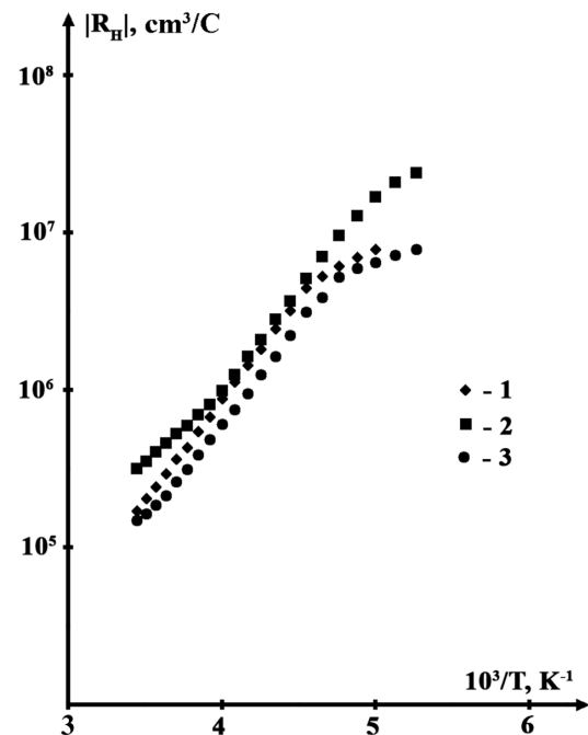
Fig. 2. Temperature dependences of the Hall constant, |R_H| = f(10^3/T) , for irradiated n -Ge single crystals at the isothermal annealing temperature T_B = 403 K and various annealing times t = 1 (1), 3 (2), and 5 h (3)
