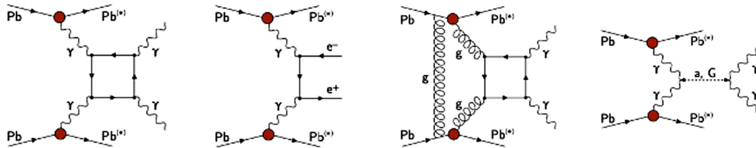
Fig. 2. Ultrapерipheral collisions at the LHC, where the impact parameter b exceeds the sum of the radii of the nuclei R_A + R_B [2]
