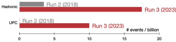
Fig. 9. Comparison of collected UPC dijet and hadronic events in Run 3 (2023) vs. Run 2 (2018) [3]
