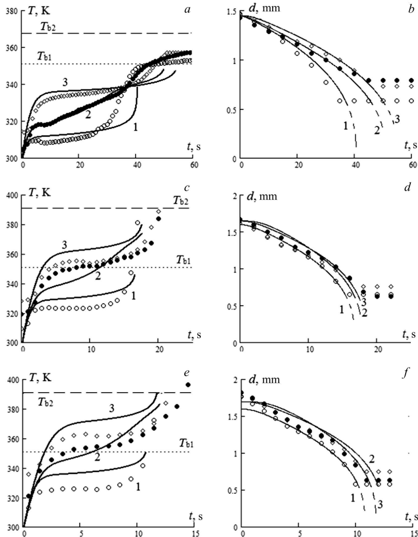
Fig. 3. Time dependences of the temperature (a, c, e) and diameter (b, d, f) of the droplets of ethanol (hollow circles), binary solution 50% ethanol + 50% butanol (solid circles), and butanol (diamonds) in air at temperatures of 368 (a, b), 485 (c, d), and 565 K (e, f). Solid curves demonstrate the results of numerical calculations taking into account heat losses through the thermocouple; symbols correspond to experimental data
