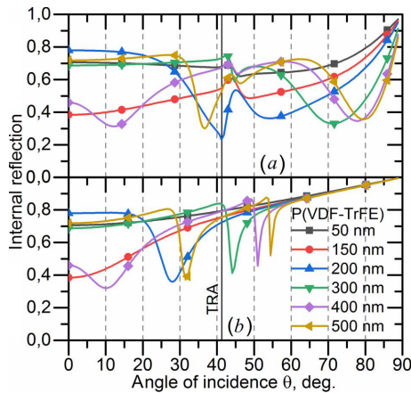
Fig. 7. ATR curves calculated for different thicknesses of the P(VDF-TrFE) layer between two 50-nm Au films. (a) – p -polarization, (b) – s -polarization. The curves are marked with symbols to distinguish them. TRA – total reflection angle
