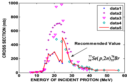
Fig. 4. The recommended cross-sections for the ^{77}\text{Se} target (present work) compared with EXFOR Library. Data 1: Ref. [24]; Data 2: Ref. [21]; Data 3: Ref. [23] Data 4: Ref. [22]; Data 5: (PW)
