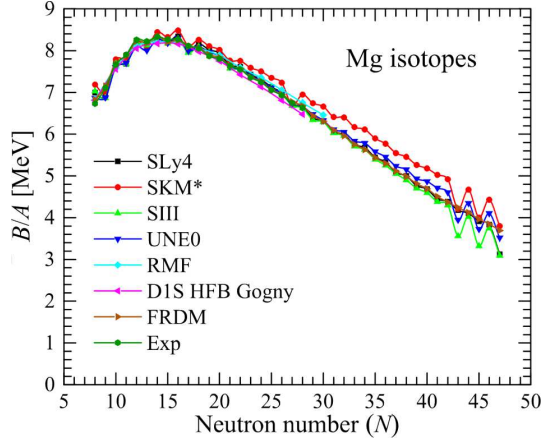
Fig. 1. (Color online) HFBTHO calculations of the B/A for even-even and even-odd Mg isotopes by using SIII, SKM*, SLy4, and UNE0 forces
