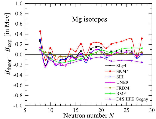
Fig. 2. (Color online) The difference between the calculated B/A and the results of FRDM [19], RMF [20], and D1S-Gogny HFB [21]
