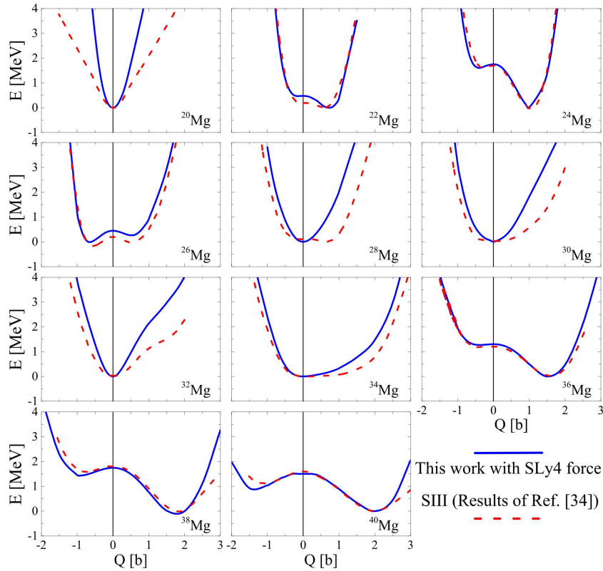
Fig. 8. (Color online) Results of HFBTHO calculations of the deformation energy curves by using the Skyrme SLy4 force for even-even ^{20\rightarrow 40}\text{Mg} isotopes in comparison with the results of Ref. [34] as a function of the axial quadrupole moment. The origin of the energy is taken at the minimum of each curve
