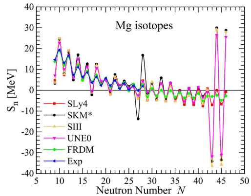
Fig. 3. (Color online) Results of HFBTHO calculations of S_n for even-even and even-odd Mg isotopes in comparison with the experimental data [18] and the data of FRDM model [19]
