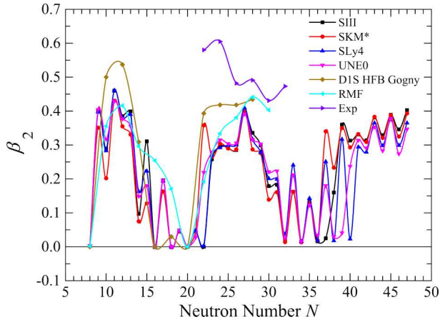
Fig. 5. (Color online) Results of HFBTHO calculations of the quadrupole deformation parameter ( \beta_2 ) for even-even and even-odd Mg isotopes in comparison with the experimental data [27], FRDM data [19], RMF data [20], and the results of D1S-Gogny HFB [21]
