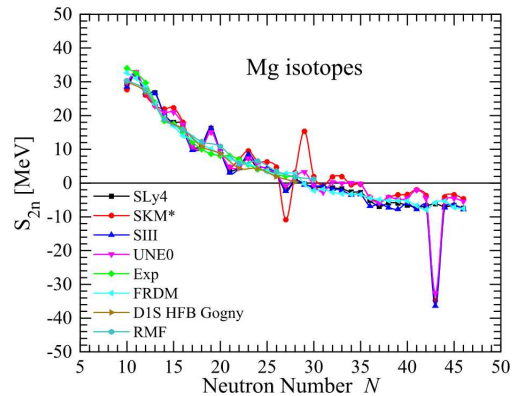
Fig. 4. (Color online) Results of HFBTHO calculations of S_{2n} for even-even and even-odd Mg isotopes in comparison with the experimental data [18], the data of FRDM model [19], the results of RMF model [20], and the data of D1S-Gogny HFB model [21]
