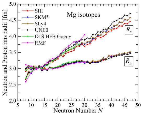
Fig. 6. (Color online) Results of HFBTHO calculations of R_n and R_p for even-even and even-odd Mg isotopes in comparison with RMF data [20] and D1S-Gogny HFB calculations [21]
