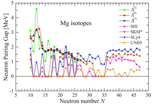
Fig. 7. (Color online) Results of HFBTHO calculations of the neutron pairing gap for even-even and even-odd Mg isotopes in comparison with difference formulas \Delta^{(3)} , \Delta^{(4)} and \Delta^{(5)} of the experimental data of AME2016 [18]
