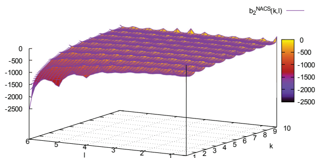
(Color online) Dependence of the second virial coefficient of non-Abelian anyons on the parameters l and k
