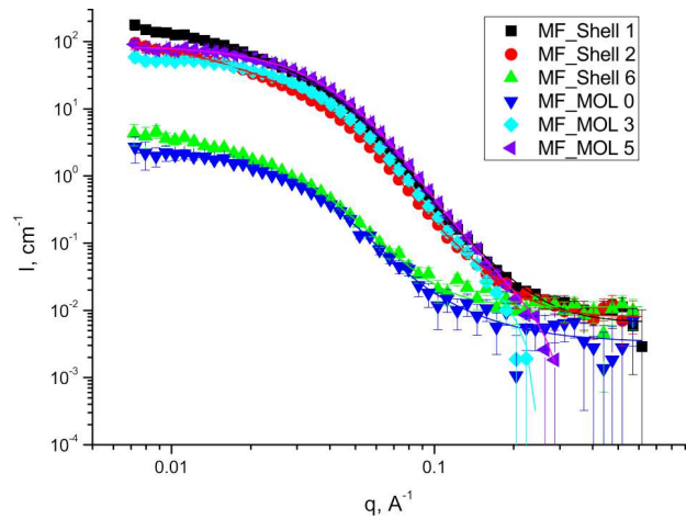
Fig. 5. SANS data (points) and the fit (curves) for the ferrofluids based on insulating transformer oils SHELL and MOL with electrodes without the dc electric field (0 kV/cm)
