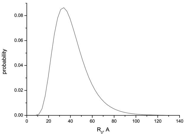
Fig. 4. Distribution of the radius of nanoparticles for the ferrofluids from SANS
