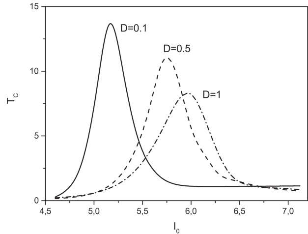
Fig. 1. Relaxation time T_C as a function of the mean value of the incident flow intensity I_0 for the various values of noise strength D and the parameters \lambda = 0.1 , Q = 0.1 , \tau_1 = \tau_2 = \tau_0 = 0.1
