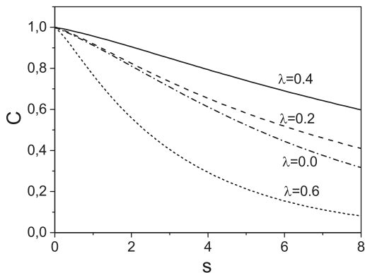
Fig. 8. Correlation function C(s) in the vicinity of the transition point ( I_0 = 5.8 ) for the various values of cross-correlation strength \lambda with the parameters D = 0.5 , Q = 0.1 , \tau_1 = \tau_2 = \tau_0 = 0.1
