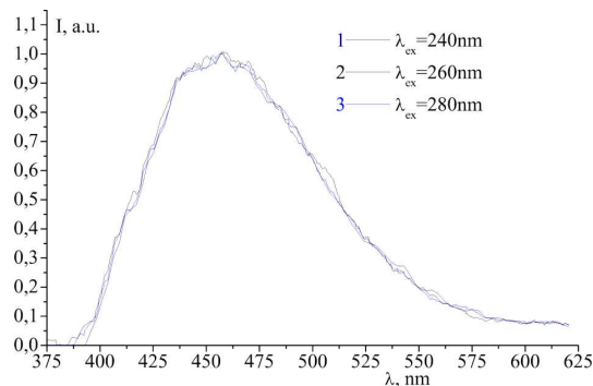
Fig. 2. Phosphorescence spectra at T = 4.2 \text{ K} of d(AGGGTTAGGGTTAGGGTTAGGG) (intact sample) excited by: \lambda = 240 \text{ nm} (1), \lambda = 260 \text{ nm} (2), \lambda = 280 \text{ nm} (3)
