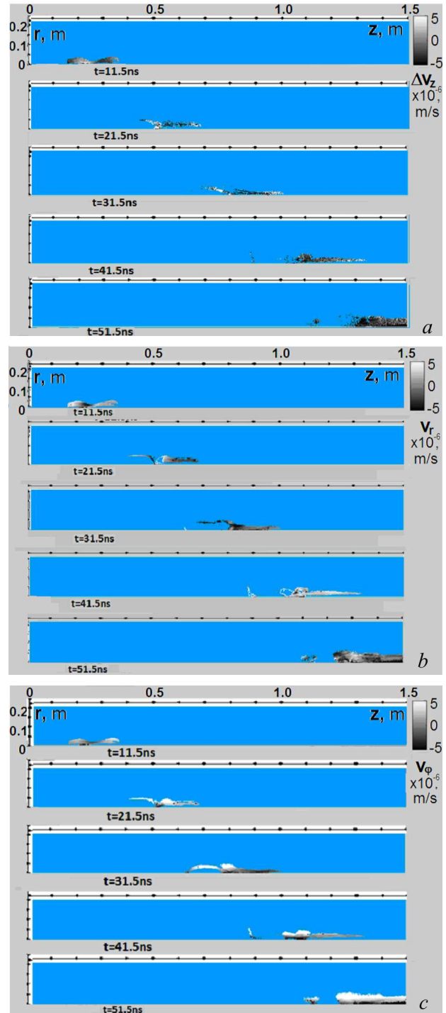
Fig. 9. Distributions of the longitudinal ( a ), radial ( b ), and azimuthal ( c ) velocity components of the bunch electrons at various stages of the bunch flight through the system ( B = 1 mT)
