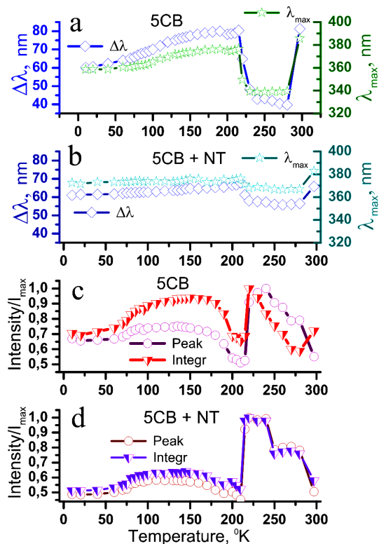
Fig. 2. Temperature dependence of the position of the band at the maximum ( \lambda_{\max} ), its half-width ( \Delta\lambda ), and peak and integral intensities (c, d) in the luminescence spectra of pure 5CB and 5CB-CNT composite
