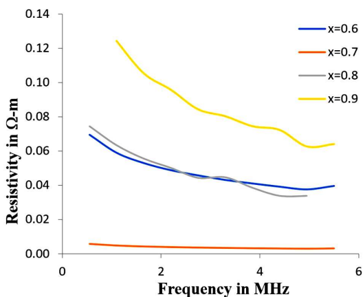
Fig. 4. Frequency-dependent resistivity for the sintered \text{Mg}_{0.25x}\text{Cu}_{0.25x}\text{Zn}(1-0.5x)\text{Fe}_2\text{O}_4 ( x = 0.6, 0.7, 0.8, 0.9 ) ferrites
