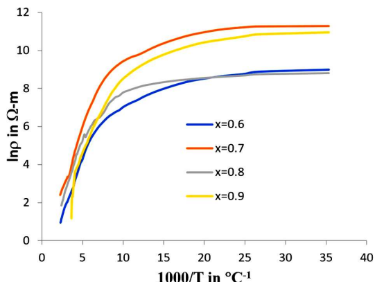
Fig. 3. Resistivity ( \ln \rho ) vs temperature ( 1000/T ) graphs of \text{Mg}_{0.25x}\text{Cu}_{0.25x}\text{Zn}(1-0.5x)\text{Fe}_2\text{O}_4 ( x = 0.6, 0.7, 0.8, 0.9 ) ferrites
