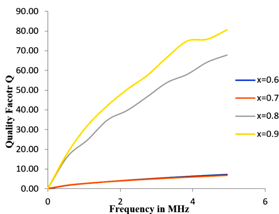
Fig. 7. Frequency-dependent quality factor for the sintered \text{Mg}_{0.25x}\text{Cu}_{0.25x}\text{Zn}(1-0.5x)\text{Fe}_2\text{O}_4 ( x = 0.6, 0.7, 0.8, 0.9 ) ferrites
