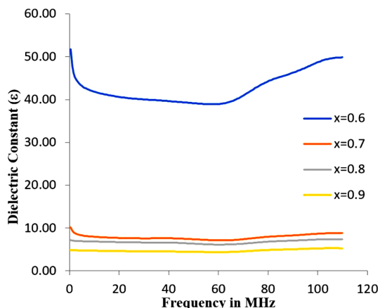
Fig. 5. Frequency-dependent dielectric constant for the sintered \text{Mg}_{0.25x}\text{Cu}_{0.25x}\text{Zn}(1-0.5x)\text{Fe}_2\text{O}_4 ( x = 0.6, 0.7, 0.8, 0.9 ) ferrites
