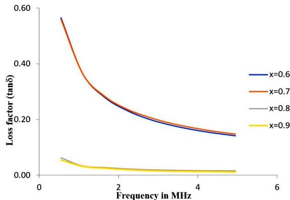
Fig. 6. Frequency-dependent dielectric loss tangent for the sintered \text{Mg}_{0.25x}\text{Cu}_{0.25x}\text{Zn}(1-0.5x)\text{Fe}_2\text{O}_4 ( x = 0.6, 0.7, 0.8, 0.9 ) ferrites
