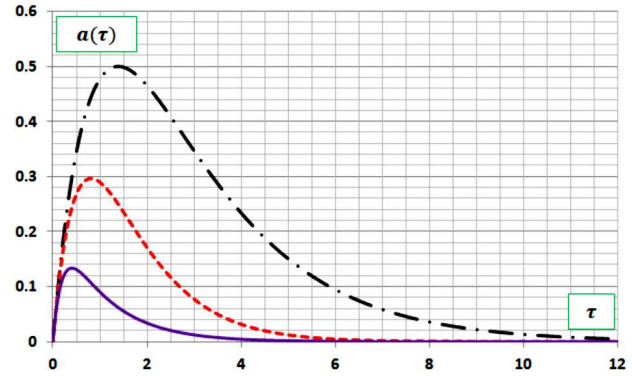
Fig. 1. Dimensionless time dependences a(\tau) of the number of activated receptors on the postsynaptic membrane for various values of the parameter \lambda = 5 (solid curve), 1.5 (dashed curve), and 0.5 (dash-dotted curve)
