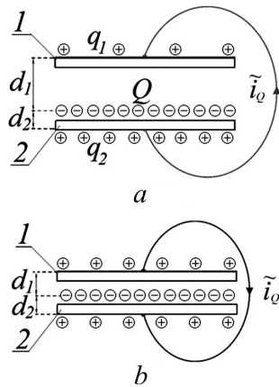
Fig. 2. Recharging the dynamic capacitor due to the motion of its plate
