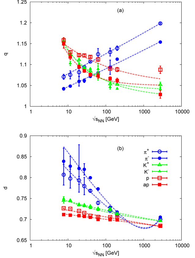
Fig. 9. (Color online) The nonextensive parameters q and d obtained from statistical fits within the Tsallis and generic axiomatic statistics, respectively, for p_T measured in A + A collisions
