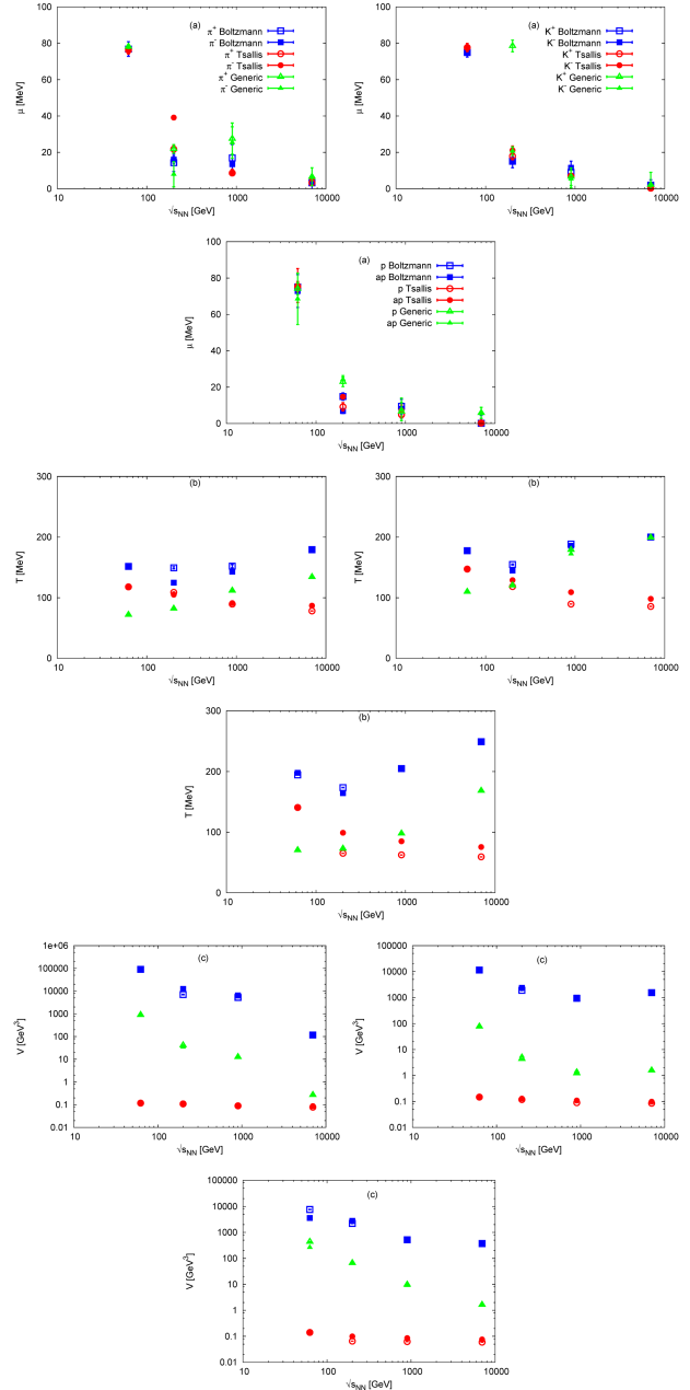
Fig. 7. (Color online) A comparison between \mu , T , and V obtained from statistical fits within the Boltzmann, Tsallis, and generic statistics for p_T measured in p + p collisions for various charged particles in a wide range of energies, compare with Fig. 4, Appendices A.2.a, A.2.b, A.2.c
