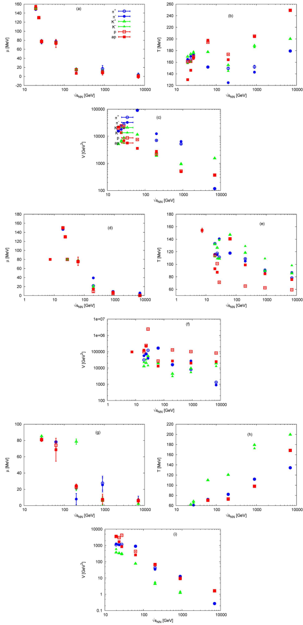
Fig. 4. (Color online) The various parameters obtained from statistical fits within the Boltzmann, Tsallis, and generic statistics for p_T measured in p + p collisions for various charged particles in a wide range of energies, Appendices A.2.a, A.2.b, A.2.c
