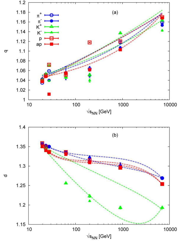
Fig. 11. (Color online) The nonextensive parameters q and d obtained from statistical fits within the Tsallis and generic axiomatic statistics, respectively, for p_T measured in NN collisions
