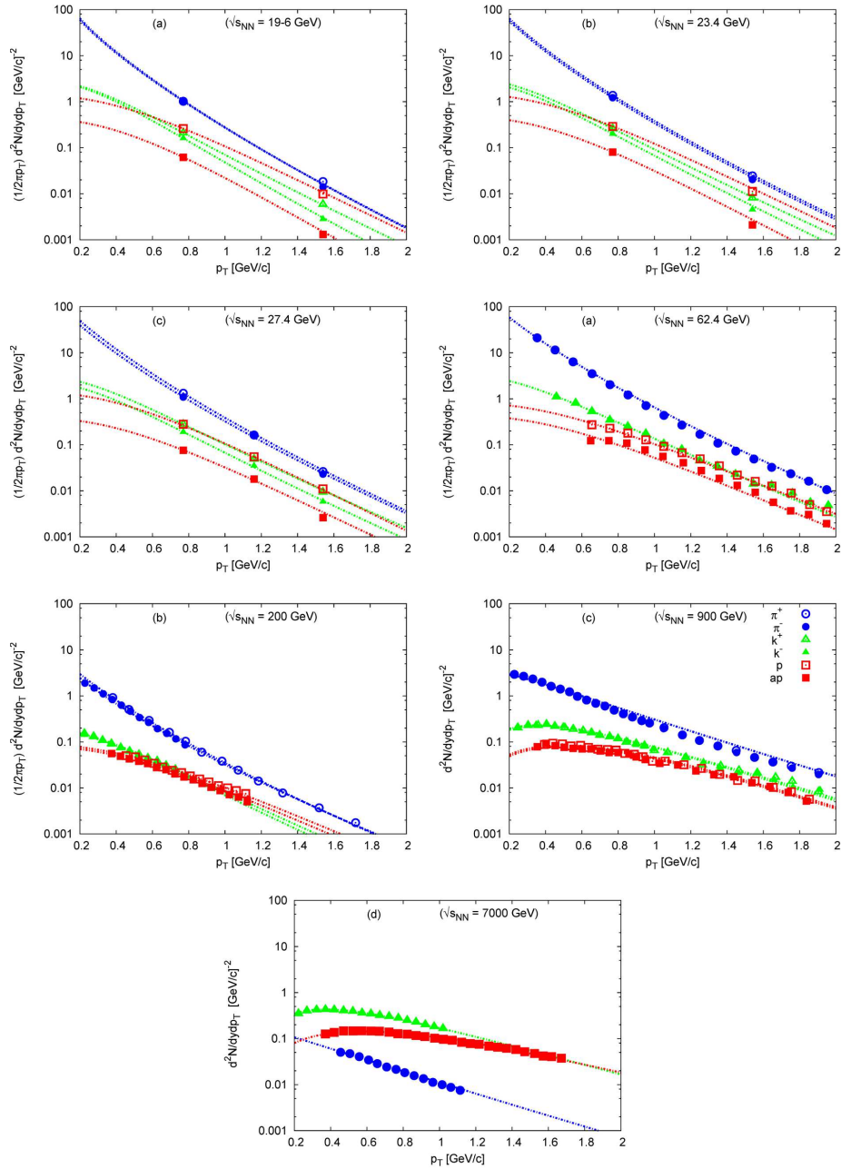
Fig. 17. (Color online) The same as in Fig. 15, but by using the generic axiomatic statistics. The corresponding fit parameters are graphed in Figs. 5 and 7
