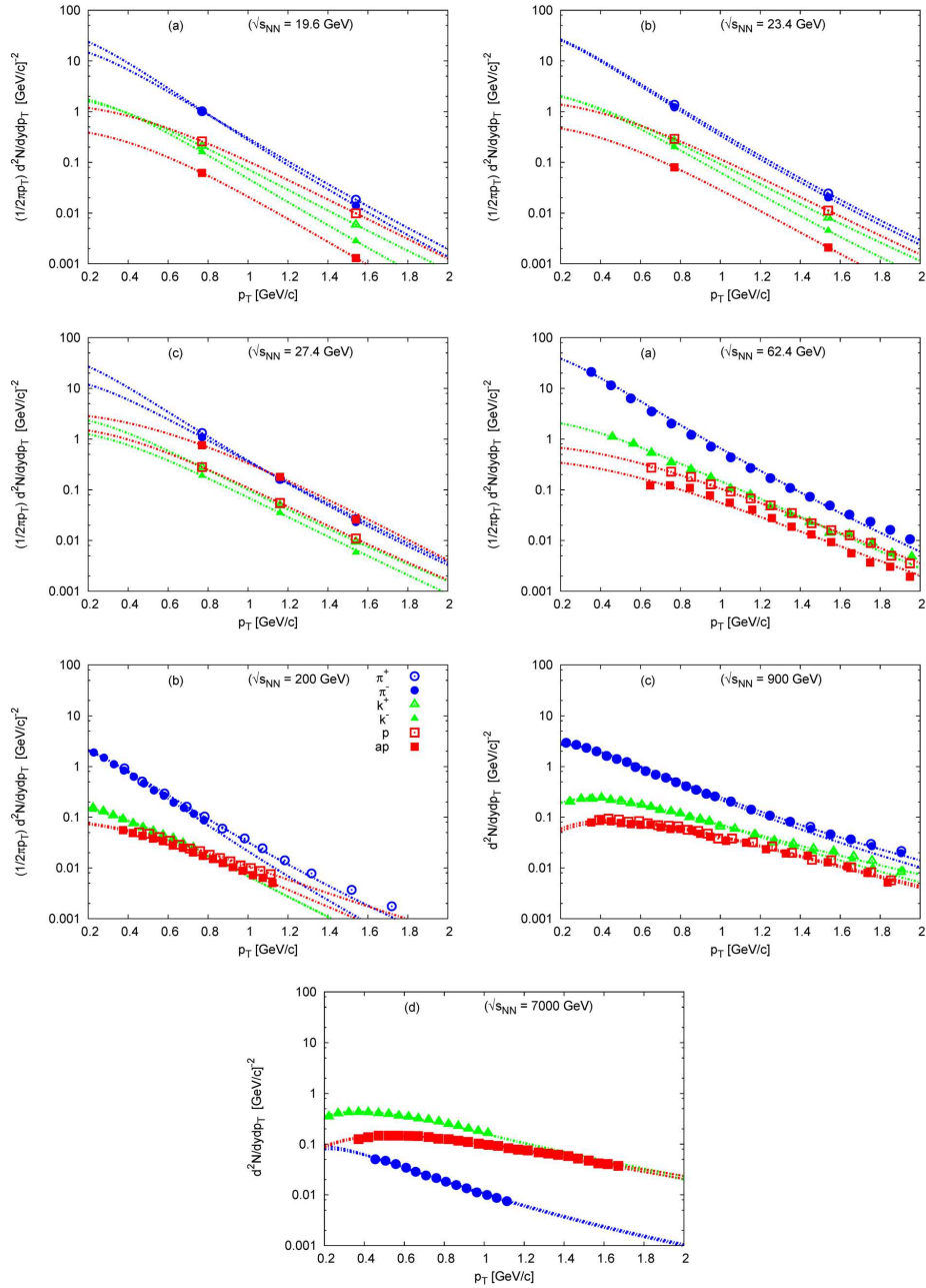
Fig. 16. (Color online) The same as in Fig. 15, but by using the Tsallis statistics. The corresponding fit parameters are given in Figs. 5 and 7
