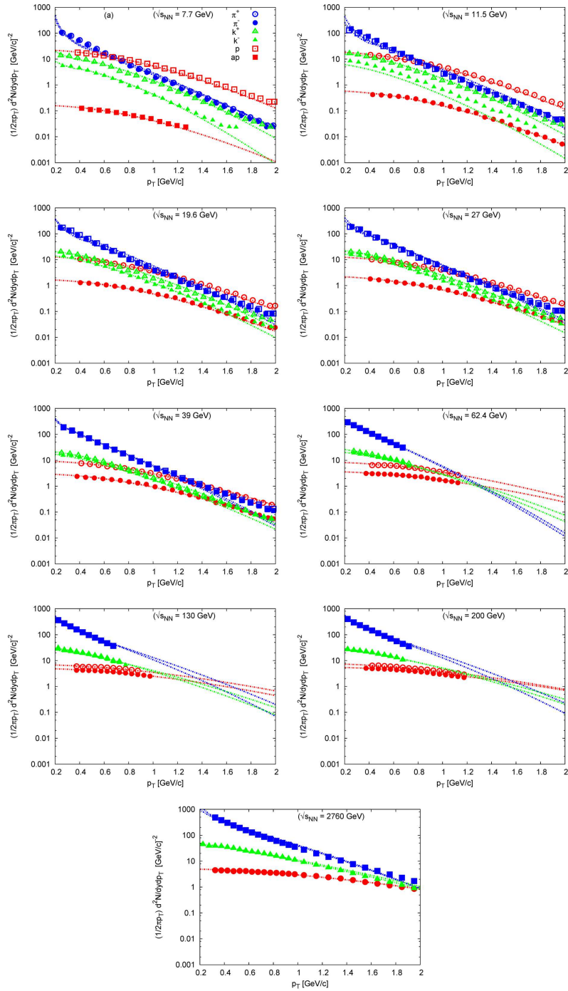
Fig. 14. (Color online) Transverse momentum spectra p_T for charged particles measured from A + A collisions at a wide range of energies (symbols) are fitted by using the generic axiomatic statistics. Panels (a)–(i) refer to the influence of changing energies from 7.7 to 11.5 to 19.6 to 27 to 39 to 62.4 to 130 to 200 GeV and to 2.76 TeV, respectively. The corresponding fit parameters are illustrated in Figs. 2 and 3
