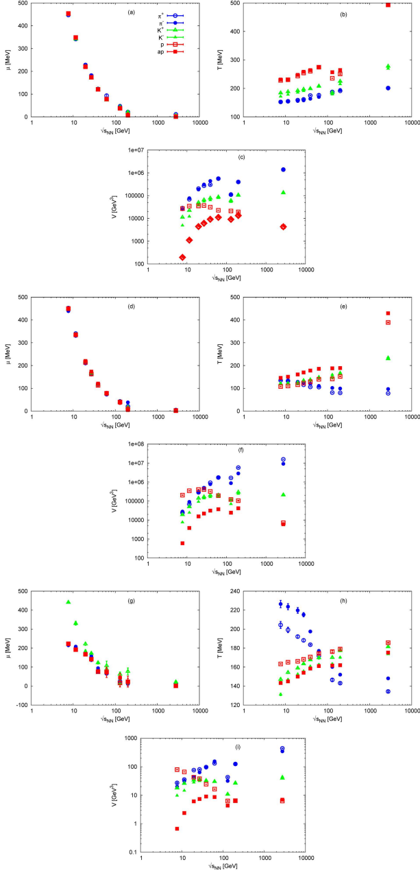
Fig. 1. (Color online) The various parameters obtained from the statistical fits within the Boltzmann, Tsallis, and generic axiomatic statistics for p_T measured in A + A collisions for various charged particles in a wide range of energies, Appendices A.1.a, A.1.b, A.1.c
