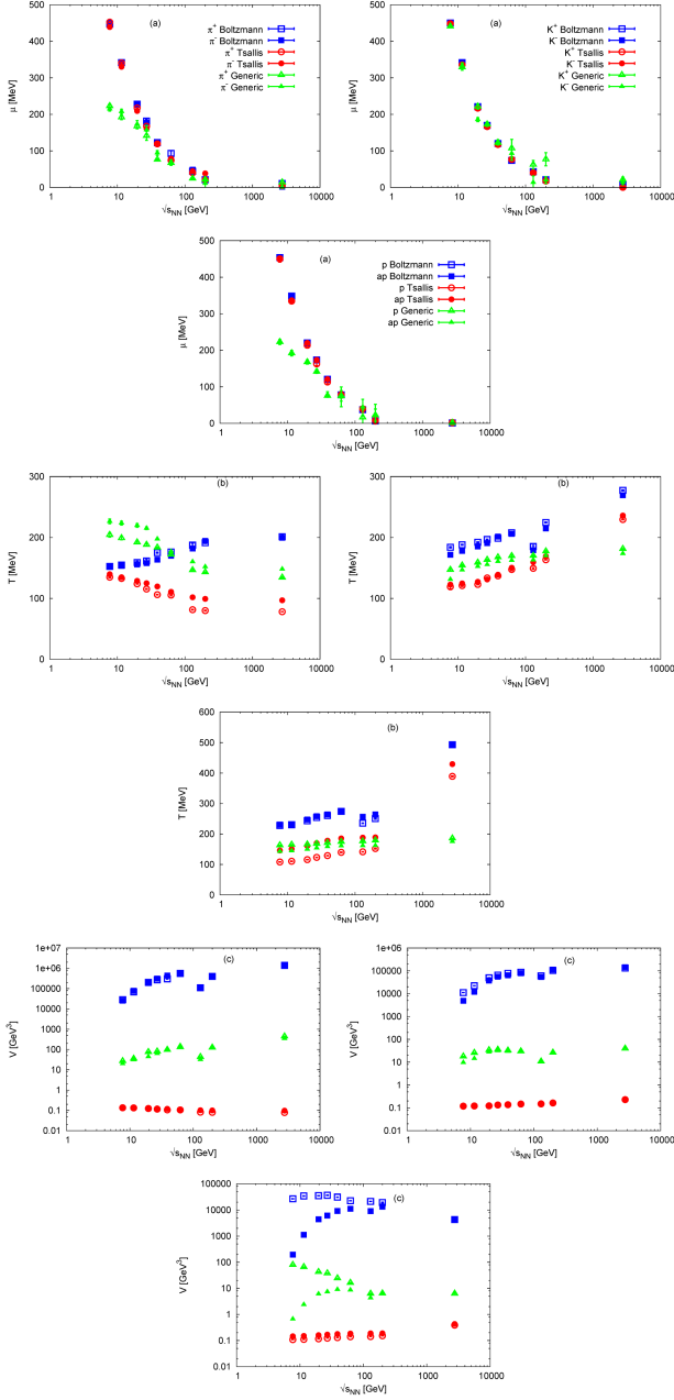
Fig. 3. (Color online) A comparison between \mu , T , and V obtained from the statistical fits within the Boltzmann, Tsallis, and generic axiomatic statistics for p_T measured in A + A collisions for various charged particles in a wide range of energies, compared with Fig. 1 and Appendices A.1.a, A.1.b, A.1.c
