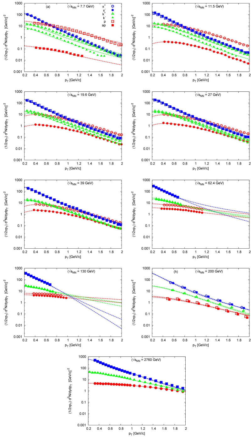
Fig. 13. (Color online) The transverse momentum spectra p_T for charged particles measured from A + A collisions at a wide range of energies are fitted to the Tsallis statistics. Panels (a)–(i) show the impacts of changing energies from 7.7 to 11.5 to 19.6 to 27 to 39 to 62.4 to 130 to 200 GeV and to 2.76 TeV, respectively. The corresponding fit parameters are illustrated in Figs. 2 and 3
