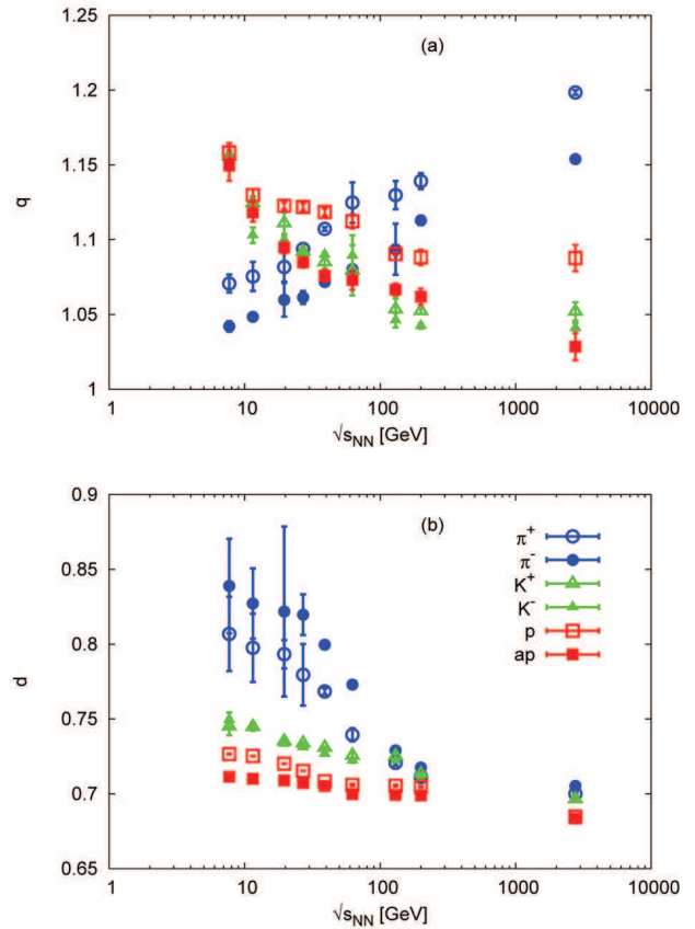
Fig. 2. (Color online) The nonextensive parameters q and d obtained from statistical fits within the Tsallis and generic axiomatic statistics, respectively, for p_T measured in A + A collisions, Appendices A.1.b, A.1.c
