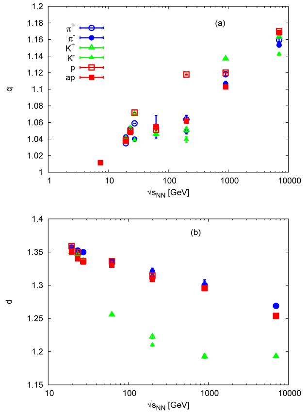
Fig. 5. (Color online) The nonextensive parameters q and d obtained from statistical fits within the Tsallis and generic axiomatic statistics, respectively, for p_T measured in p + p collisions, Appendices A.2.b, A.2.c
