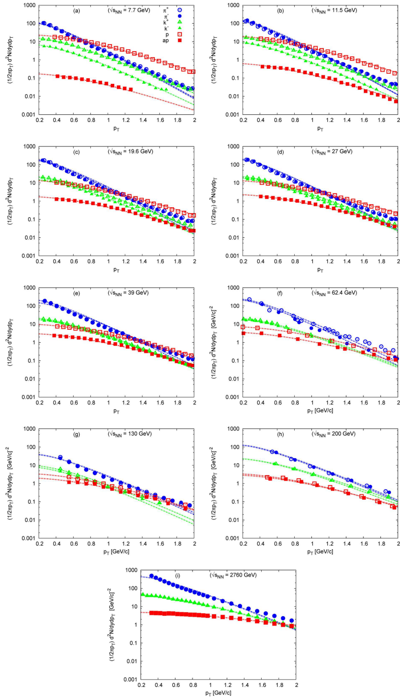
Fig. 12. (Color online) The transverse momentum spectra p_T for charged particles measured from A + A collisions in a wide range of energies are analyzed by using the Maxwell–Boltzmann statistics. Panels (a)–(i) refer to the change in the center-of-mass energies from 7.7 to 11.5 to 19.6 to 27 to 39 to 62.4 to 130 to 200 GeV and to 2.76 TeV, respectively. The fit parameters are shown in Fig. 3
