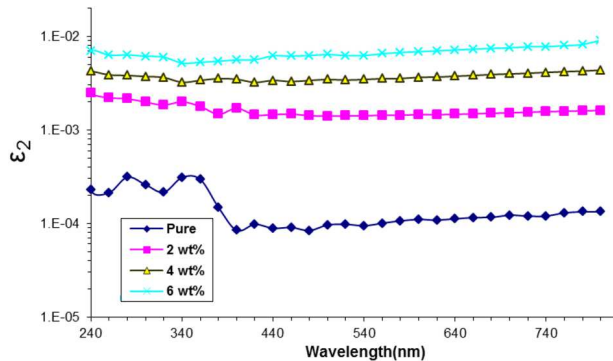
Fig. 9. Variation of the imaginary part of the dielectric constant for (PVA-MnO 2 -ZrO 2 ) nanocomposite with the wavelength
