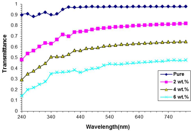
Fig. 2. Variation of the transmittance for (PVA-MnO 2 -ZrO 2 ) nanocomposite with the wavelength
