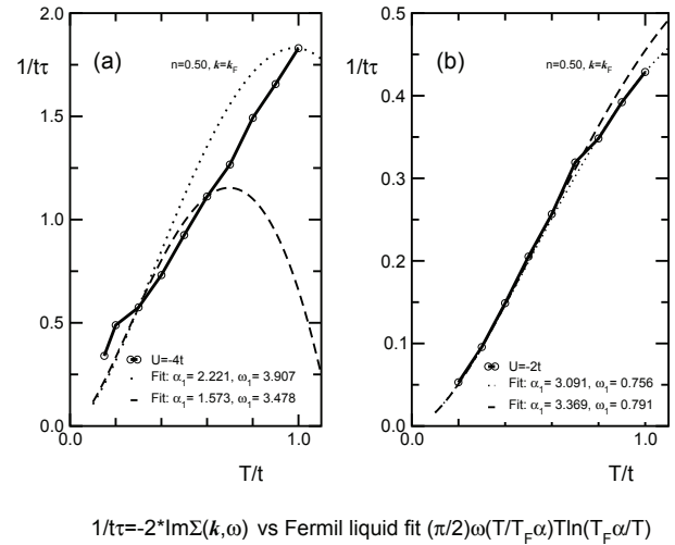
Fig. 7. Marginal temperature dependence of the lifetime of a Landau quasiparticle as compared to the 2D Fermi liquid picture (see the text)
