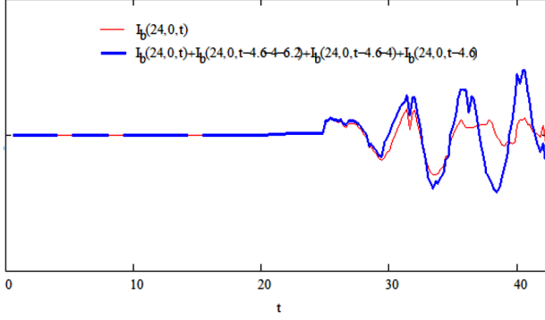
Fig. 1. The red line represents a change in the wave potential over time for a single generated wave, while the blue line depicts a change in the wave potential over time for four generated waves, as described in formula (20)
